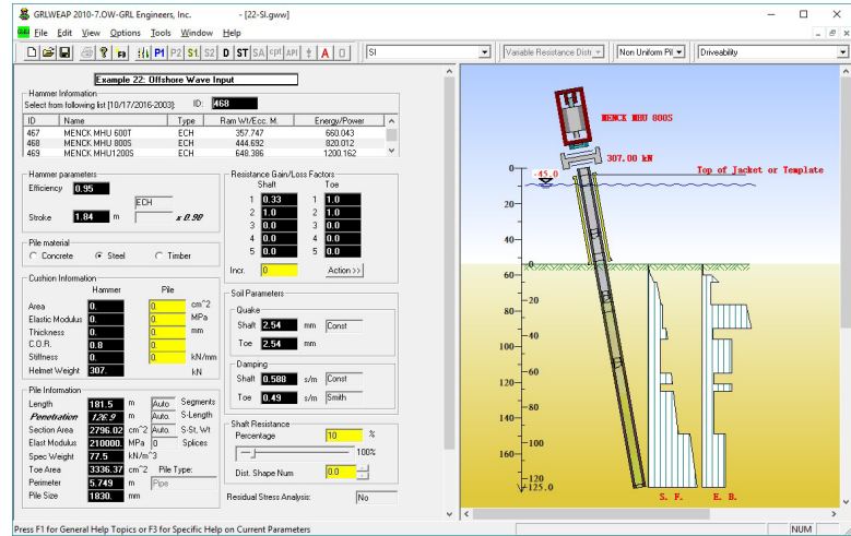
GRLWEAP Main Input Screen
